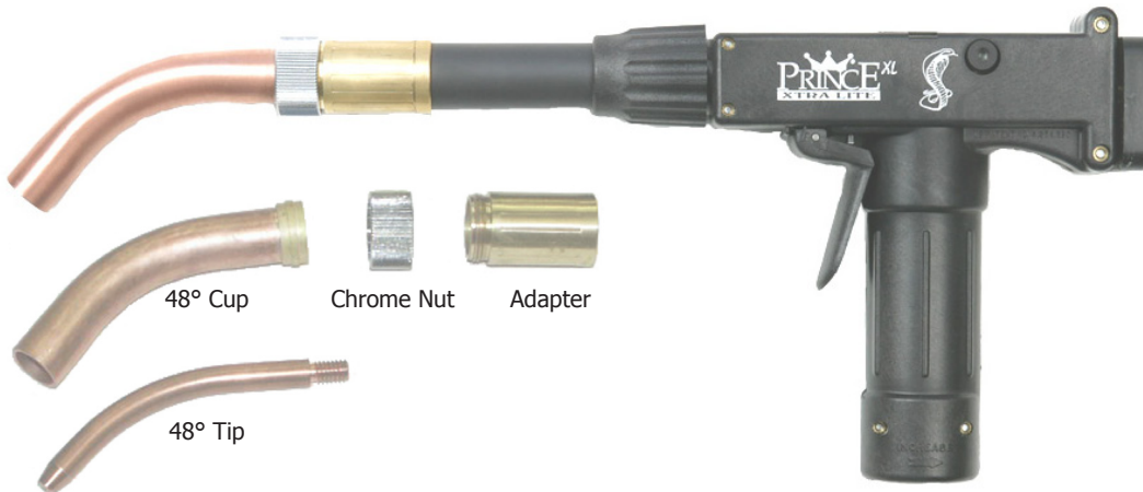
48° Curved Cup, Chrome Nut and Adapter shown assembled on a Straight Air/Water Barrel on a Prince XL.
